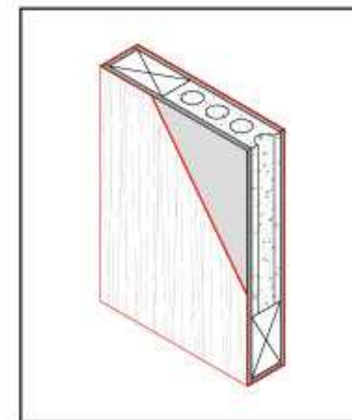
Tubular chipboard core
