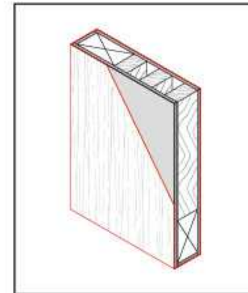
Semi solid core
