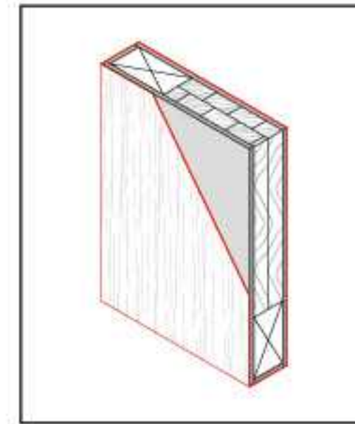
Staved lumber core
